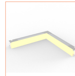
L shape light in connector Order Code: AC05 Dimension: 100×100×12.5mm/ 3.94"×3.94"×0.49"(L×W×H) Material: aluminium
